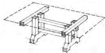
Trestle
