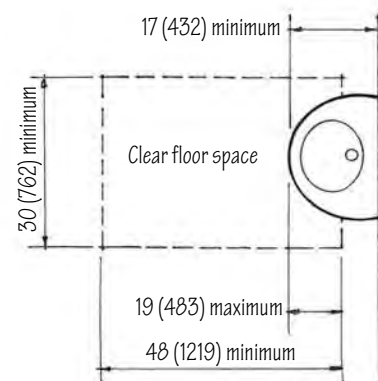
Accessible lavatory
