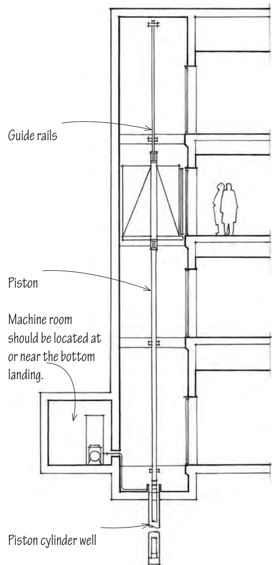
Hydraulic Elevator
