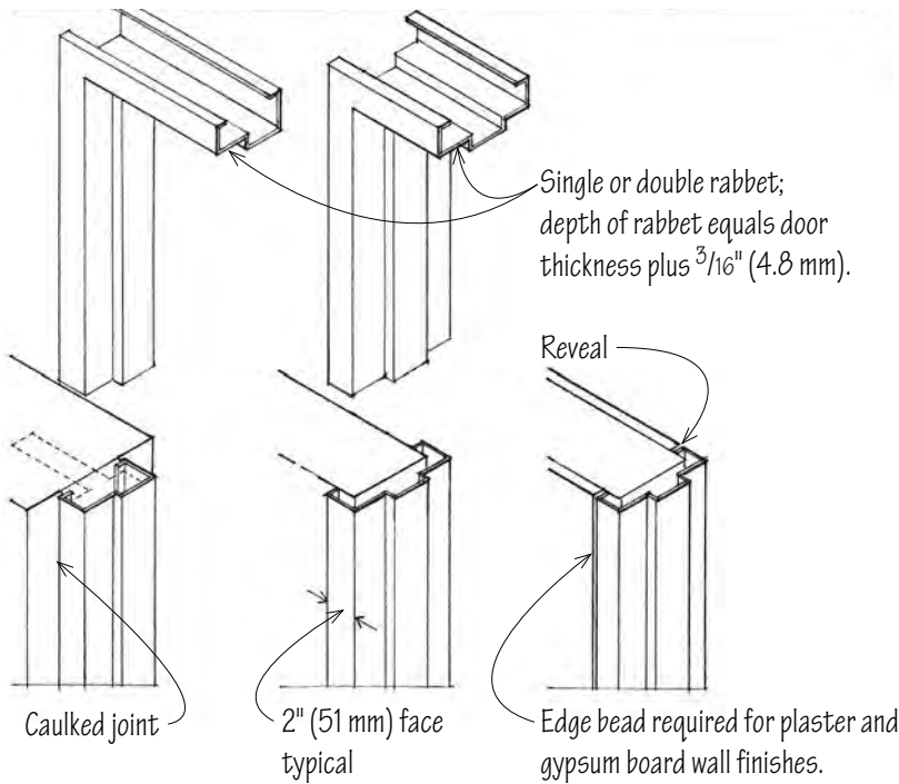
Butt Condition at Masonry Wall
