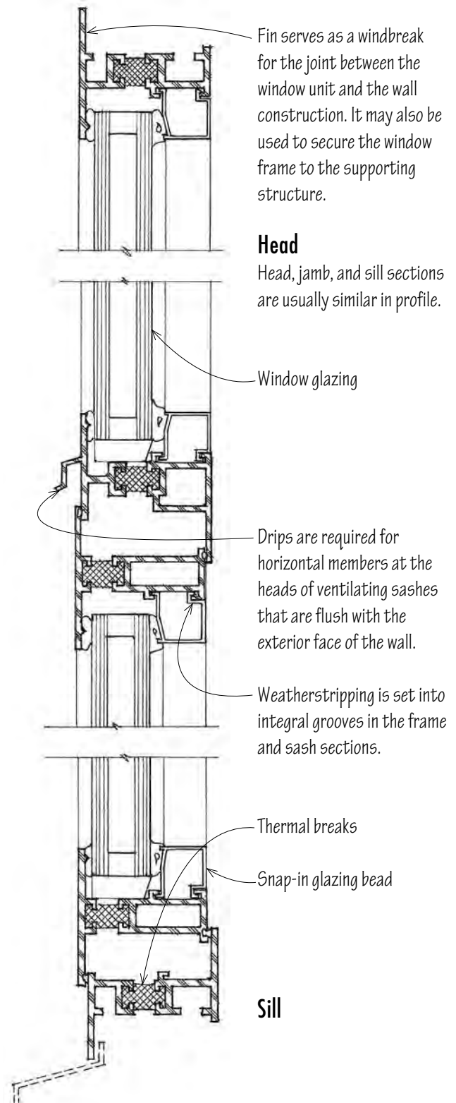
Typical Metal Window
