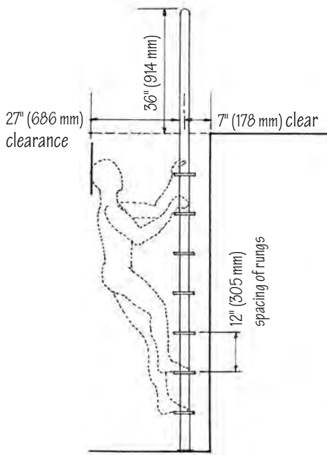
Ladders
