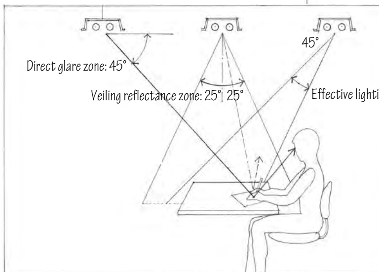
Bright, concentrated light sources above and forward of the task surface can cause veiling reflectances.
