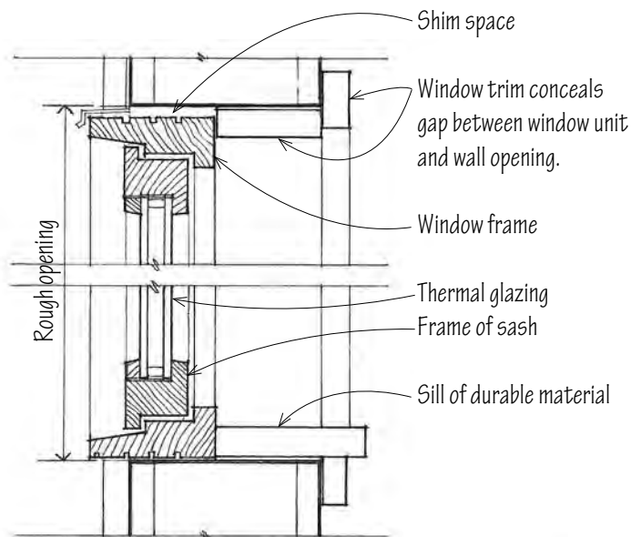
Section Through a Typical Window
