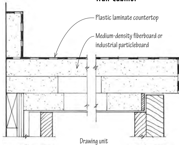
Wall Cabinet
