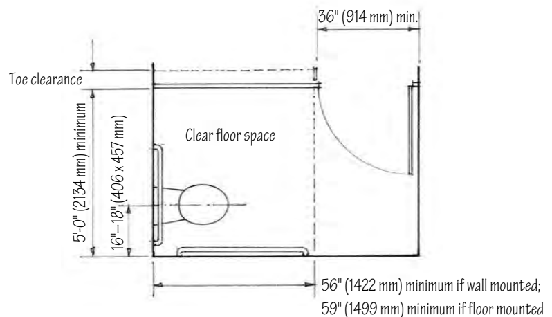
Accessible End Toilet Stall
