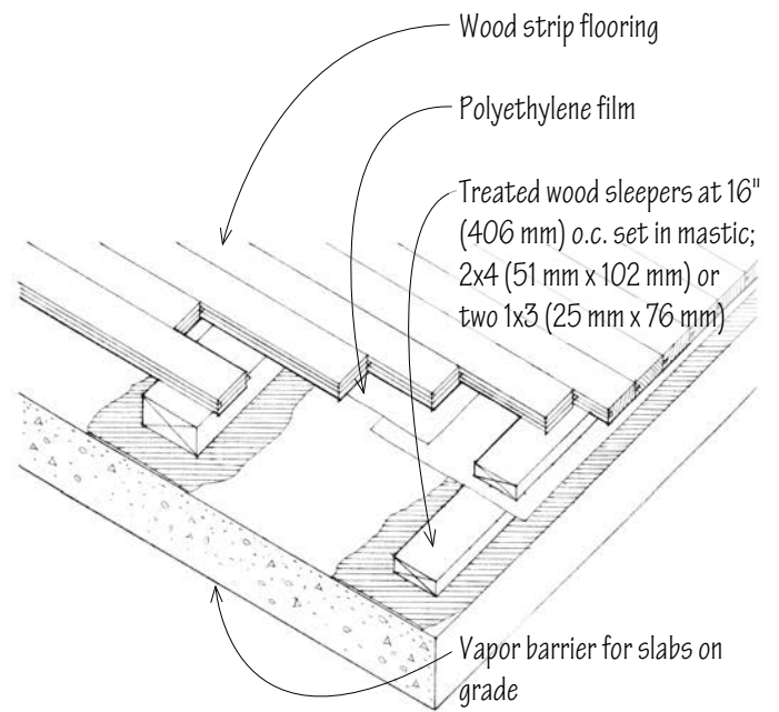
Wood Flooring over a Concrete Slab
