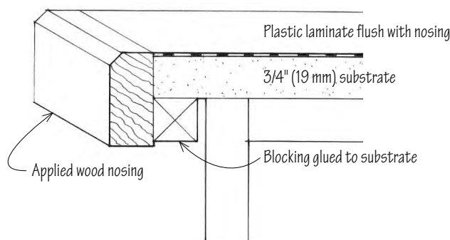
Countertop Nosings
