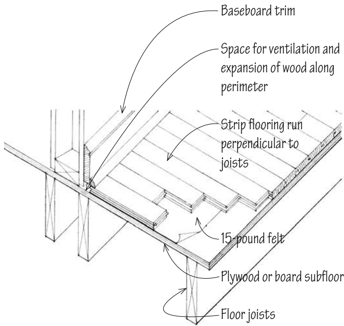
Wood Flooring over a Subfloor and Joists
