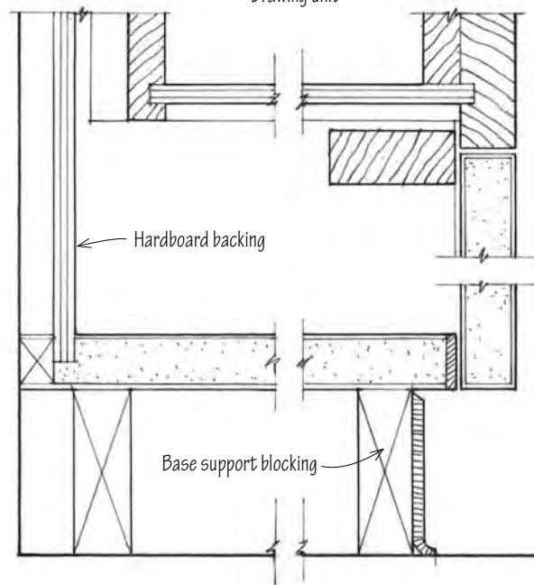
Base Cabinet
