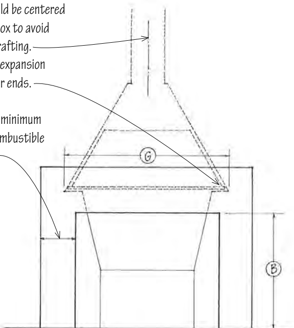
Fireplace Elevation
