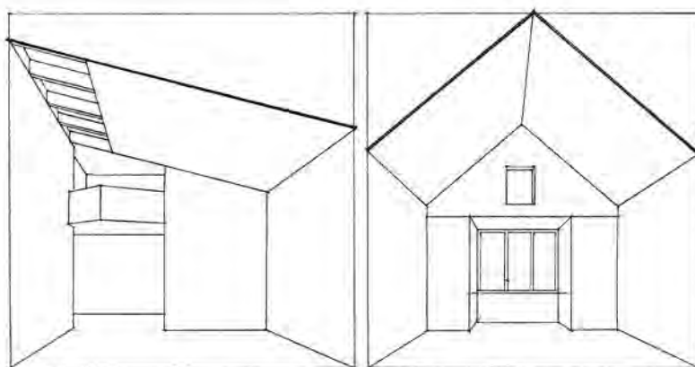
Single-slope ceiling
