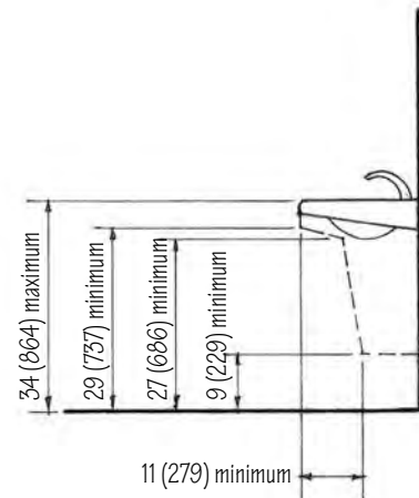
Accessible lavatory
