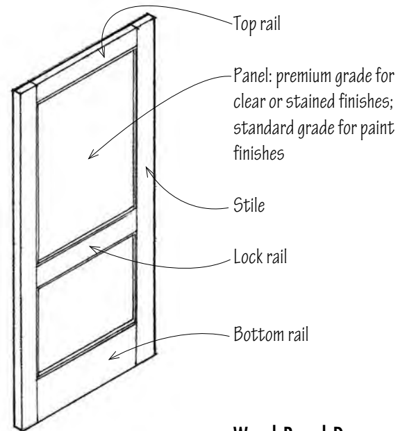
Wood Panel Doors
