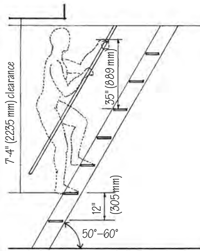
Ship's Ladders
