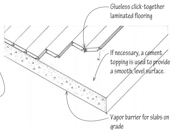
Glueless Laminated Wood Flooring Installation
