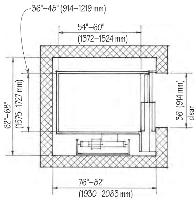
LU/LA Elevator
