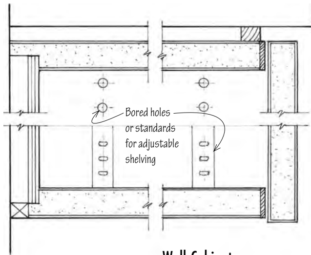
Wall Cabinet
