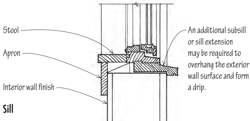
Typical Wood Window
