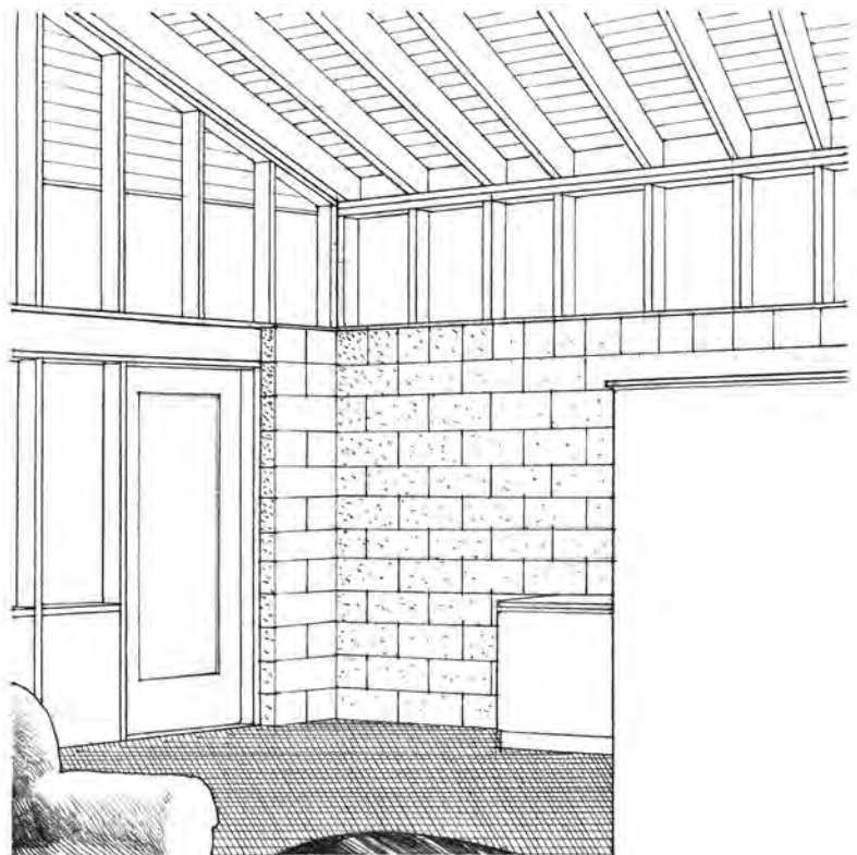
Texture can also result from the manner in which materials are assembled in construction.
