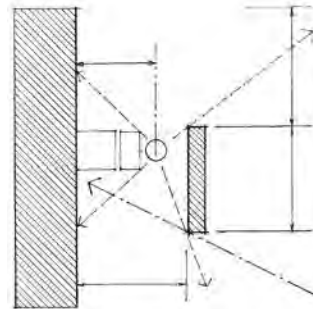
Valance lighting directs the light upward and/or downward from a light source concealed by a horizontal board or band.
