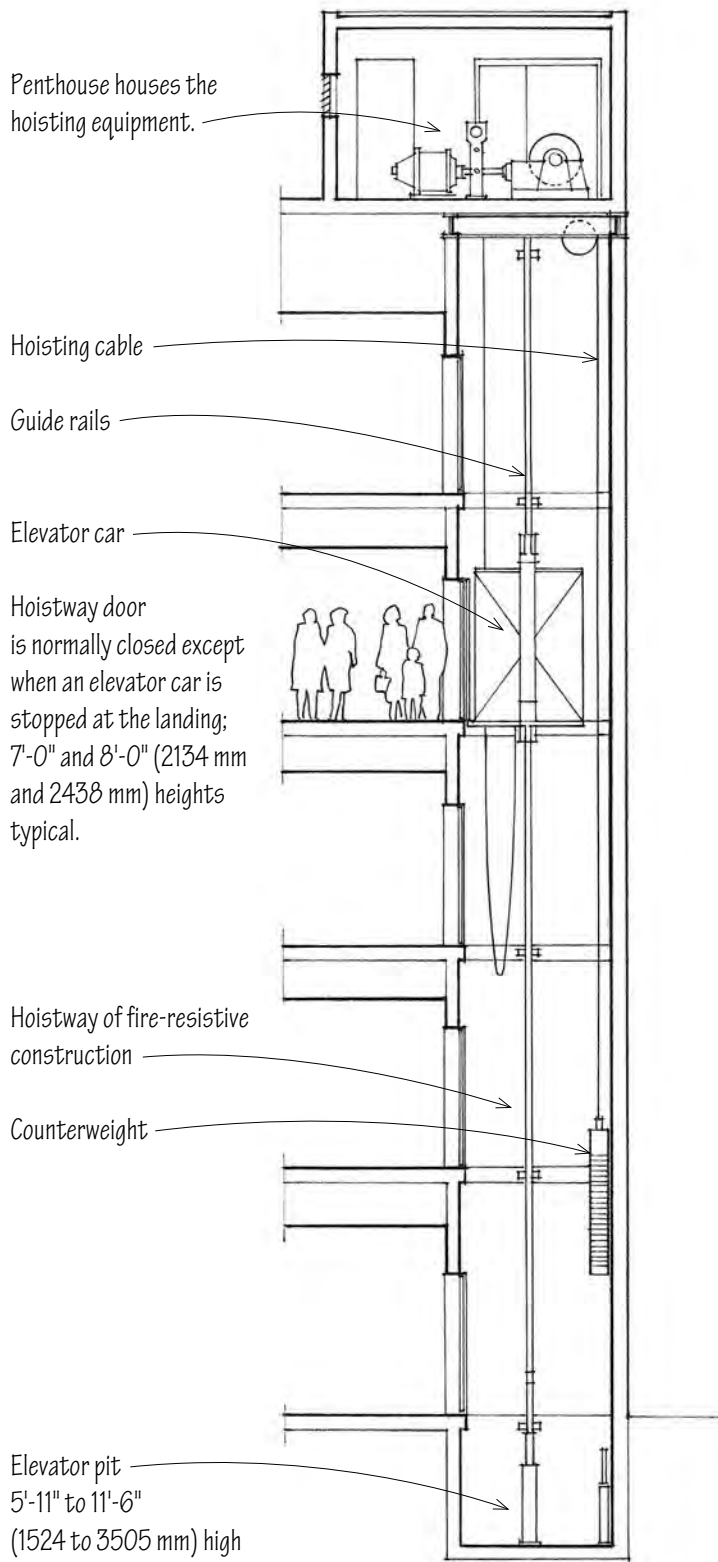
Traction Elevator
