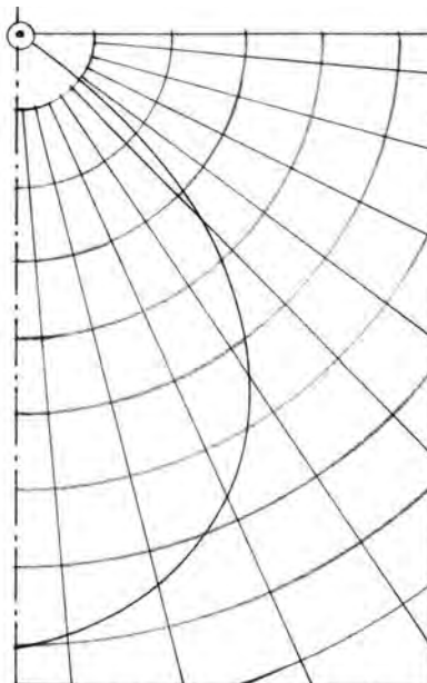
Luminous-intensity distribution curve of a light fixture
