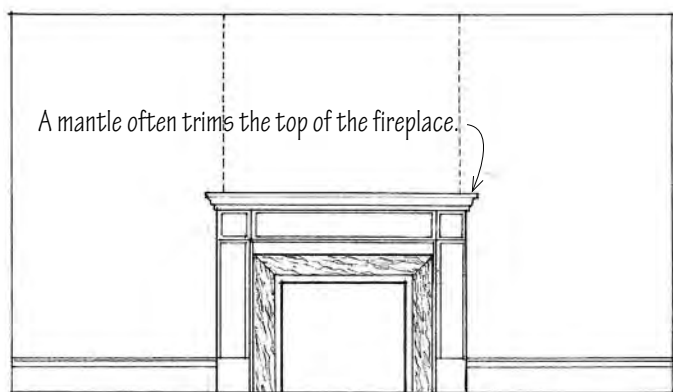
No woodwork is permitted within 6" (152 mm) of the fireplace opening.
