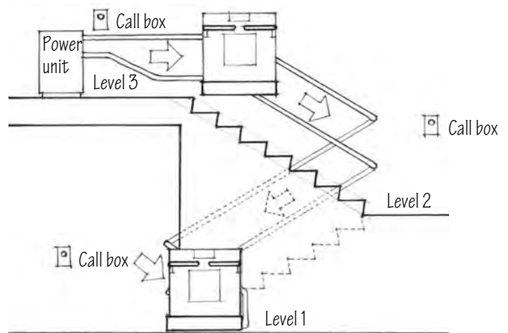
Inclined Wheelchair Lift
