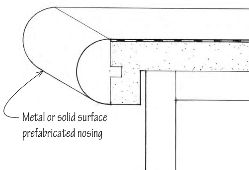
Countertop Nosings
